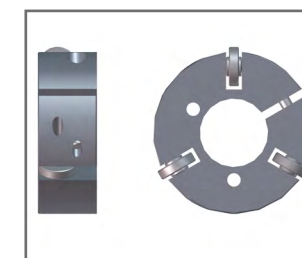
Centering guide with rollers 69-78,5 mm Order No.0657948 77,5-97 mm Order No. 0657949
