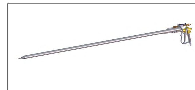
Hand lance with gun 1800 mm long Order No. 0656948
