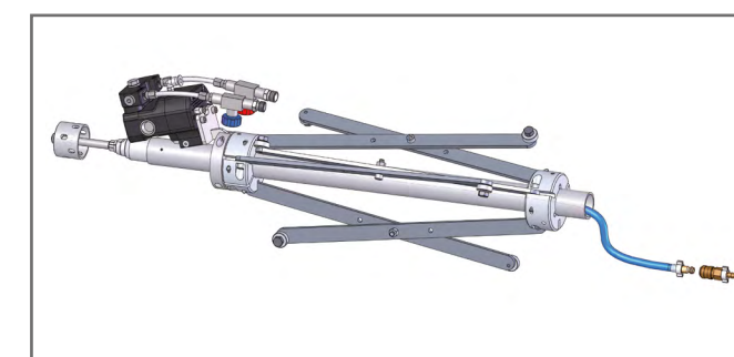
PU 4040 Automatic Gun for internal pipe coating with Polyurea Order No. 0659289 • Guide ø 210- ø 400 mm (Larger dia. upon request)
